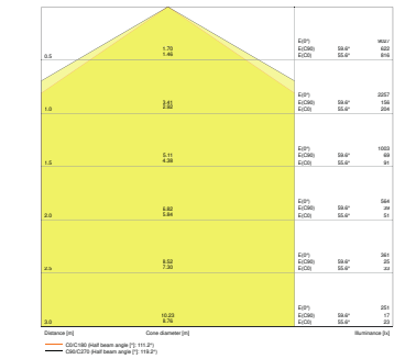
TRUSYS PFM 50W 4000K VW 4x1 EUE LEDV
