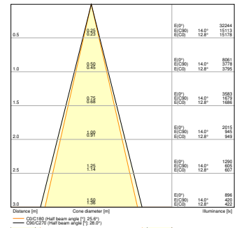
TR SP ZOOM DIM P 30W 93040 WT 4000K 21D
