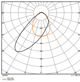
TRUSYS FLEX P 35W 840 WW CL WT
