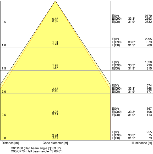
DL_UGR19_DN195_PFM_21W840_DALI_WT
