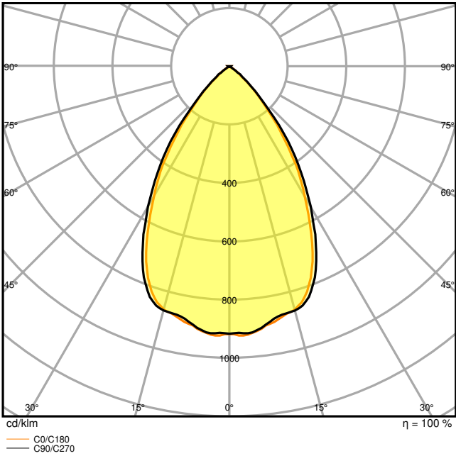
DL_UGR19_DN195_PFM_21W840_DALI_WT
